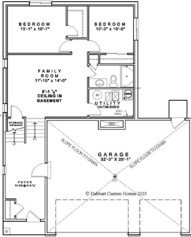
The Ava - Lower Level
