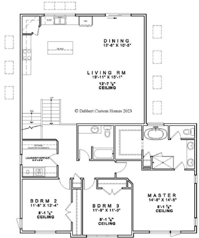
The Ava - Upper Level w/ Alt. Kitchen Layout/Master Bath Layout
