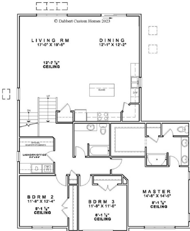
The Ava - Upper Level w/ Pocket Office Layout
