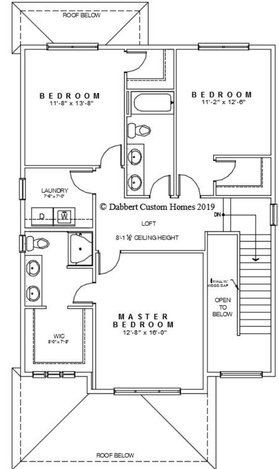
THE ROCHELLE 2.0 UPPER LEVEL
