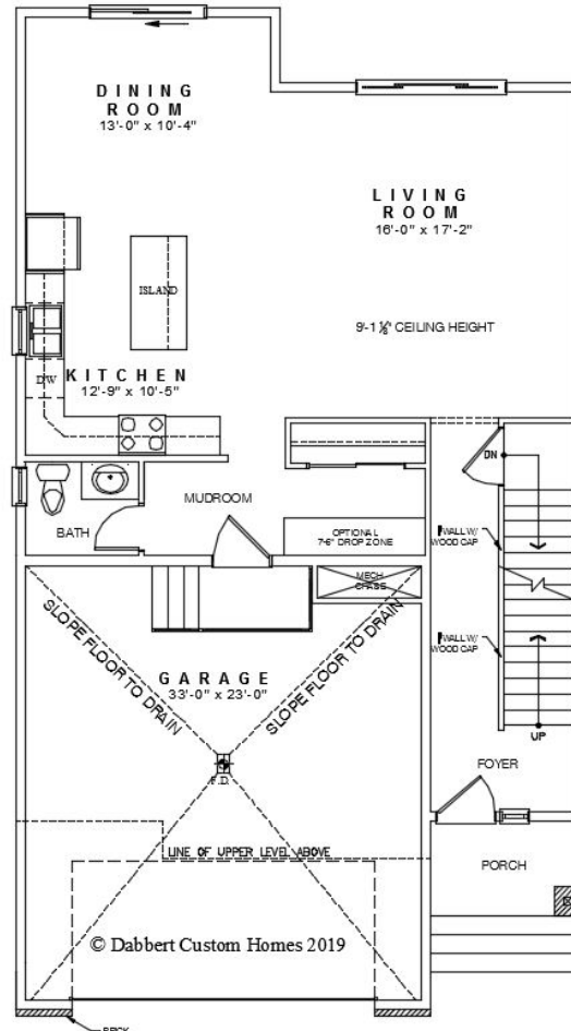
THE ROCHELLE 2.0 MAIN LEVEL
