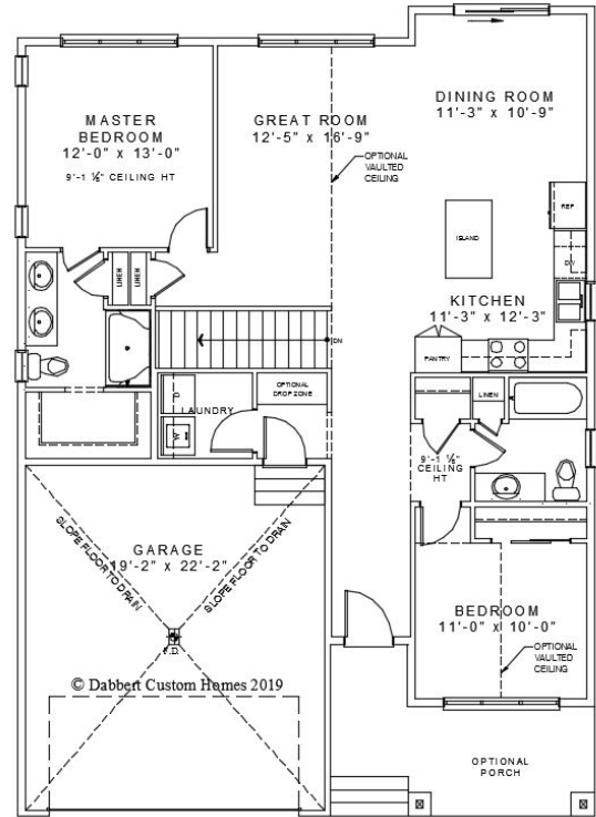
THE MAGGIE 2.0 MAIN LEVEL
