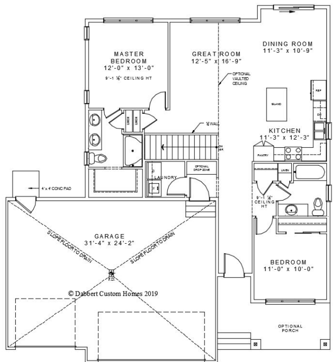
THE MAGGIE 3.0 MAIN LEVEL
