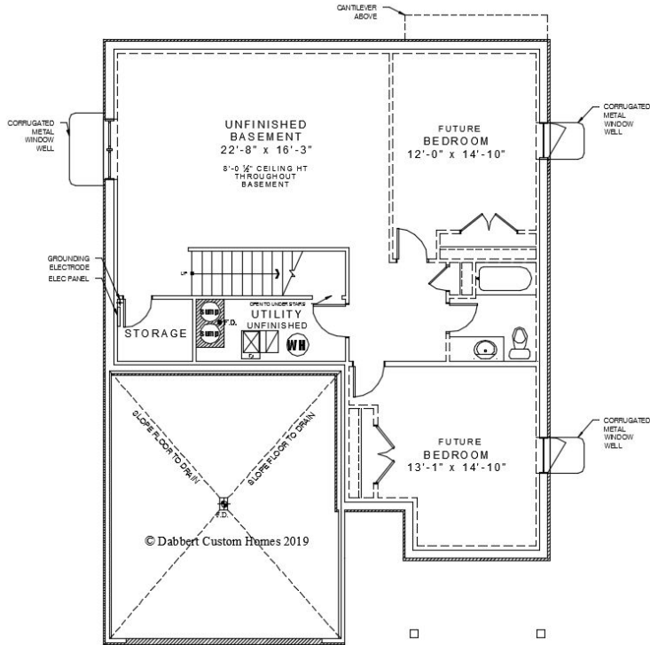
THE MAGGIE 2.0 LOWER LEVEL
