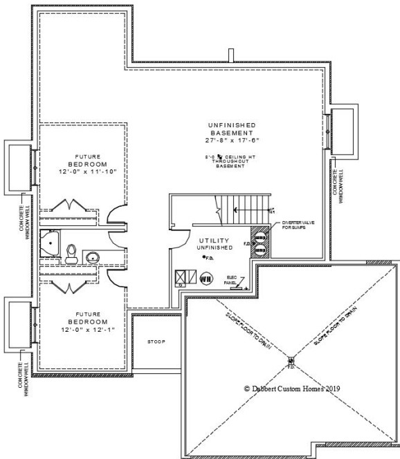
THE LILLIAN 3.0 LOWER LEVEL
