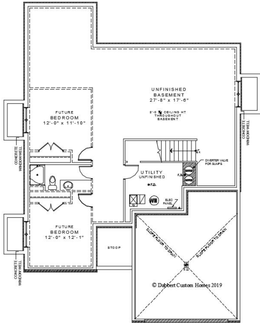
THE LILLIAN 2.0 LOWER LEVEL
